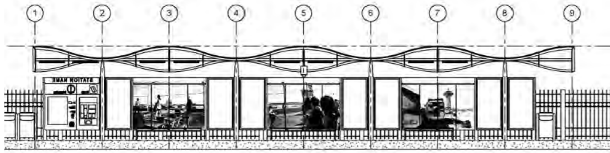
CONVENTION CENTER SOUTHBOUND ELEVATION CONT. SCALE: 1/4" = 1'-0"
